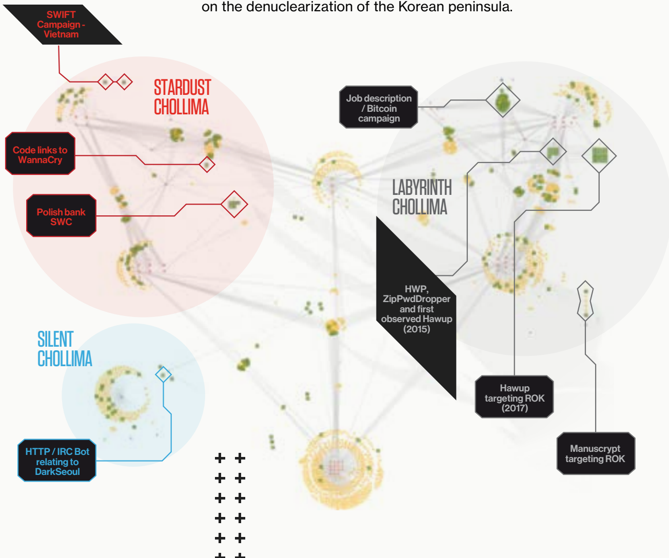
Figure 14. Clustering DPRK Adversaries Based on Code Blocks
